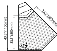
45° Interior Counter FRN-CI45
