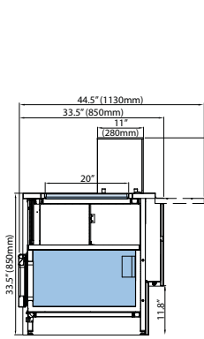
Refrigerated w/storage, FRTRT
