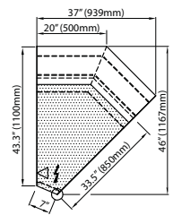
45° Exterior Counter FRN-CE45
